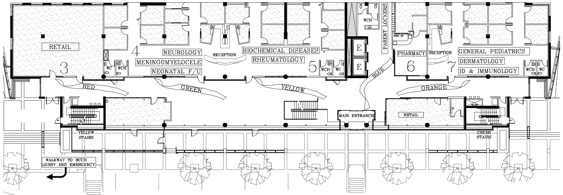
First floor (Level 1)
